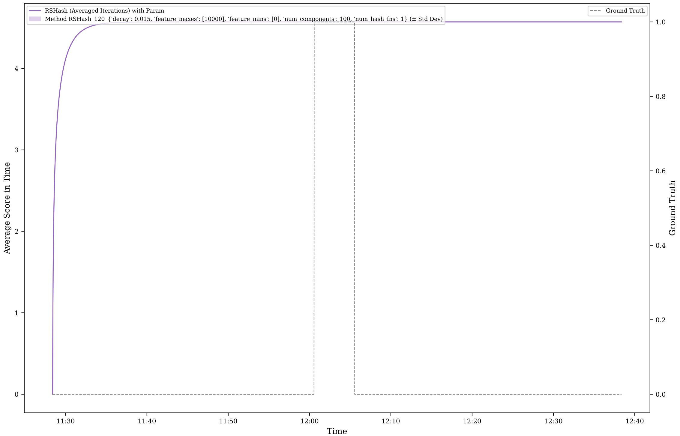
Method RSHash Score for Scenario A8
